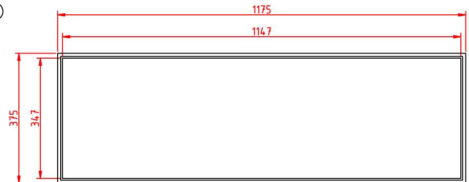
TOP VIEW OPEN
