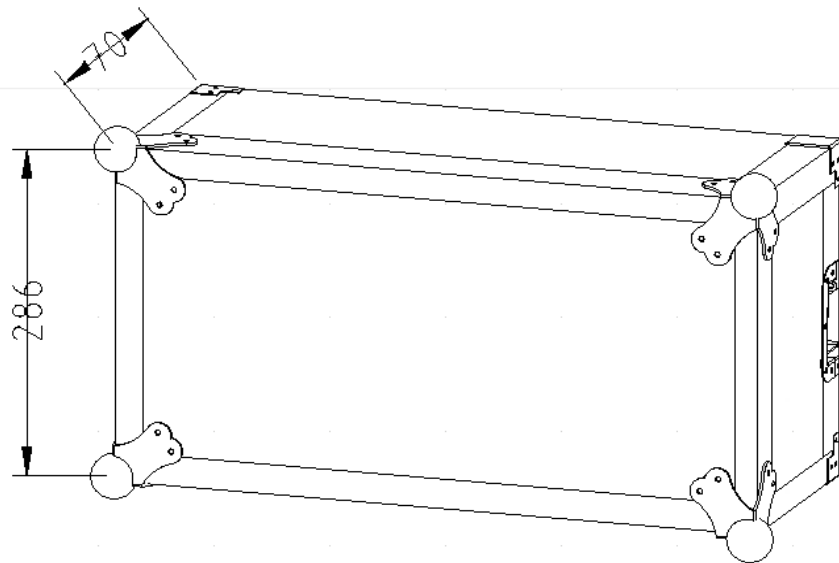
Cobra Case: FC182 Material: Ply Wood Dimensions in mm, May Vary Slightly.
