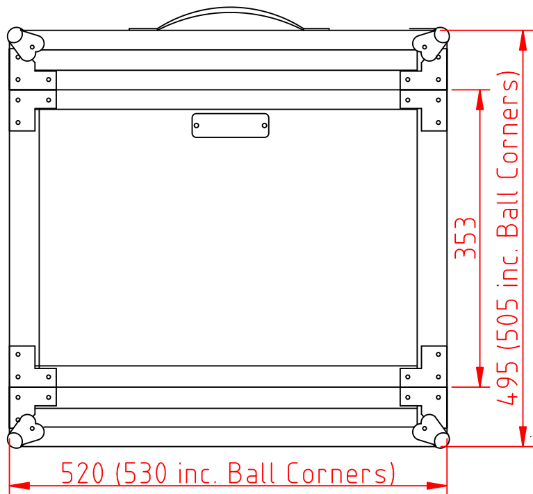
Cobra Case - FC149 19" 2U Rack Case 350mm Deep Material: Plywood Dimensions in mm, may vary slightly
