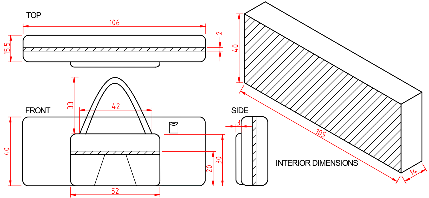
Cobra Case Keyboard Bag CC1050 Material: Nylon Zips: No10 Dimensions in cm, may vary slightly
