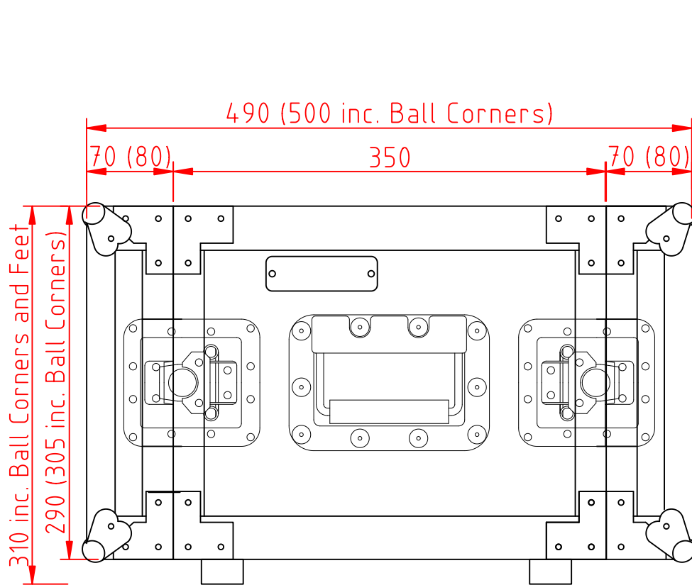
Cobra Case - FC151 19" 6U Rack Case 350mm Deep Material: Plywood Dimensions in mm, may vary slightly
