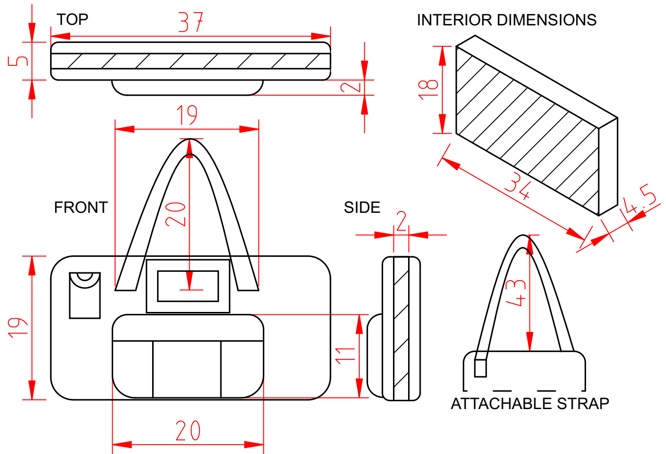
Cobra Case Equipment Bag CC1086 Material: Polyester 600d Zips: No8 Dimensions in cm, may vary slightly
