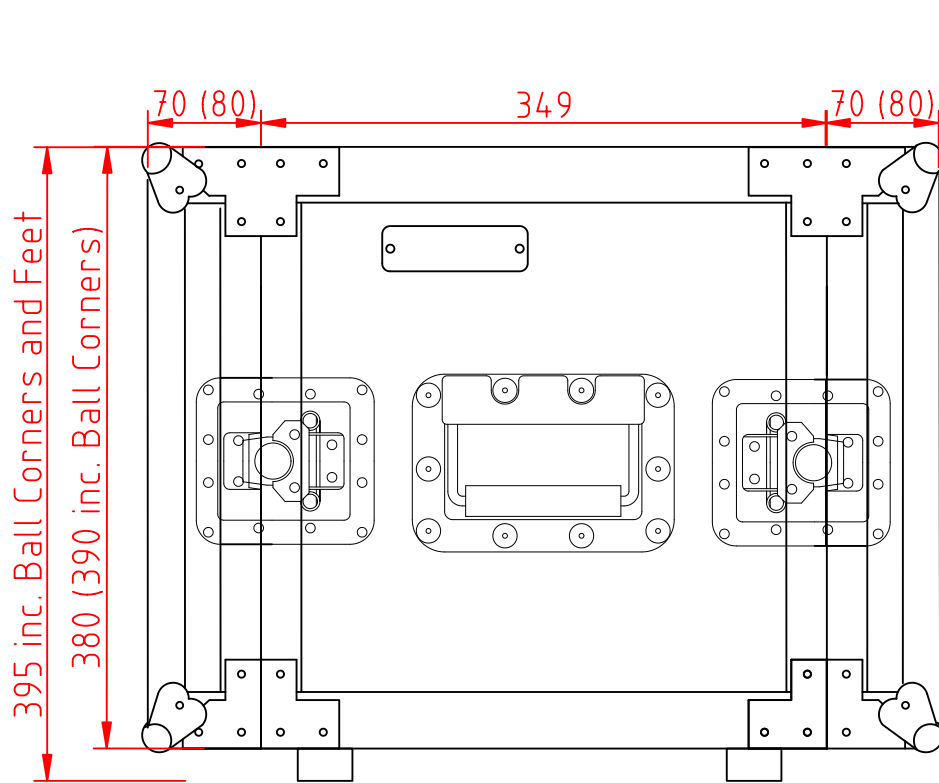
Cobra Case - FC152 19" 8U Rack Case 350mm Deep Material: Plywood Dimensions in mm, may vary slightly
