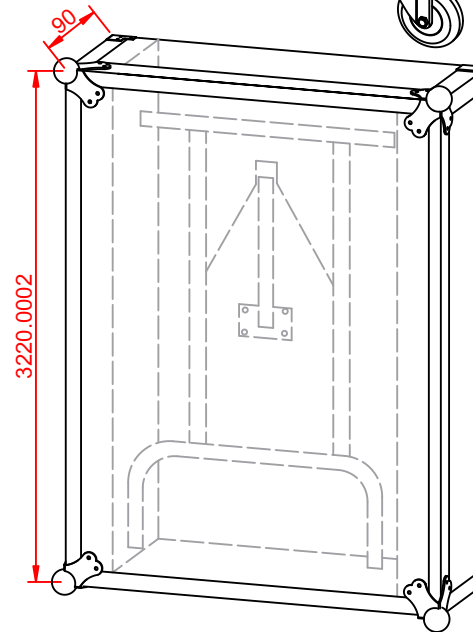
Cobra Case - FC67 Universal Drawer Case with Table Material: Plywood Dimensions in mm, may vary slightly
