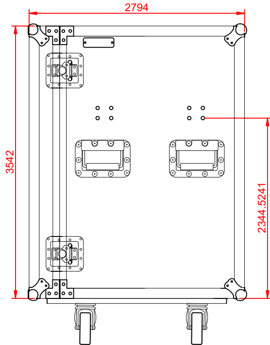
Cobra Case - FC67 Universal Drawer Case with Table Material: Plywood Dimensions in mm, may vary slightly
