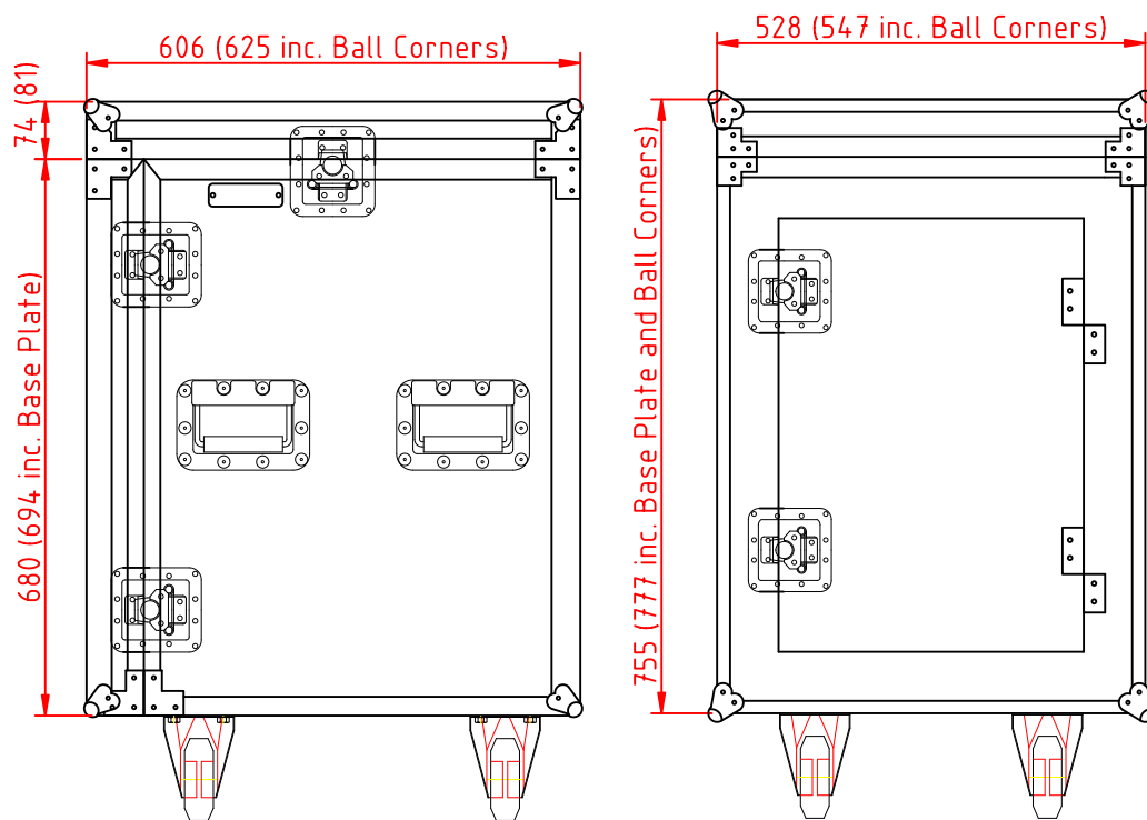
Cobra Case - FC69 Rack Flight Case with 10U Sloping Top and 12U Bottom Material: Plywood Dimensions in mm, may vary slightly
