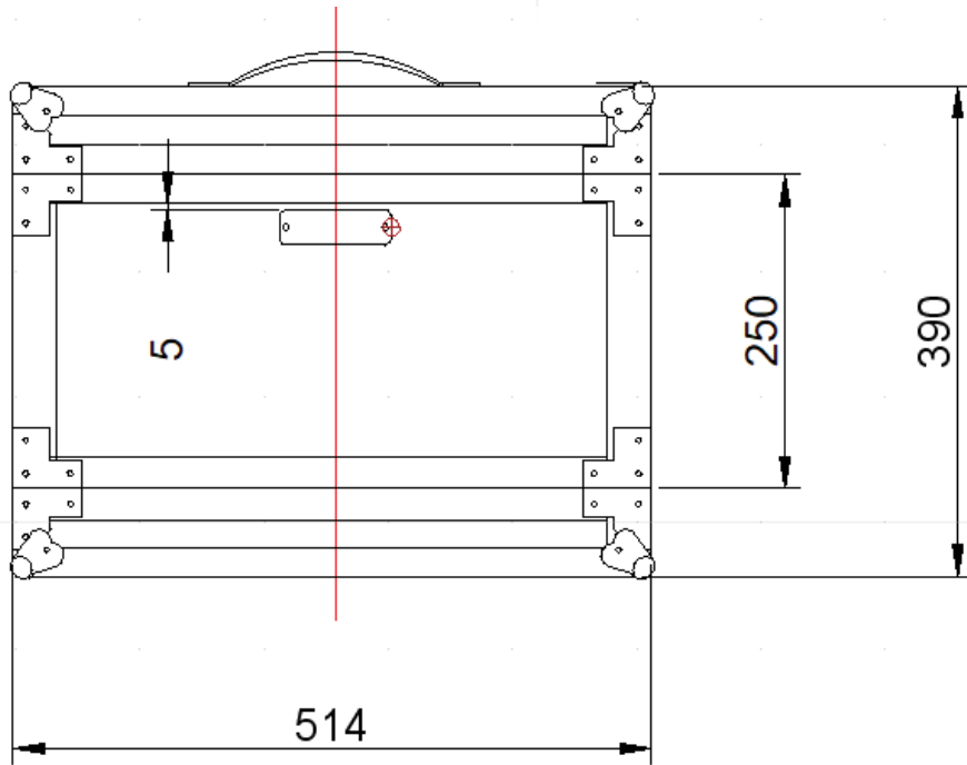
Cobra Case: FC180 Material: Ply Wood Dimensions in mm, May Vary Slightly.
