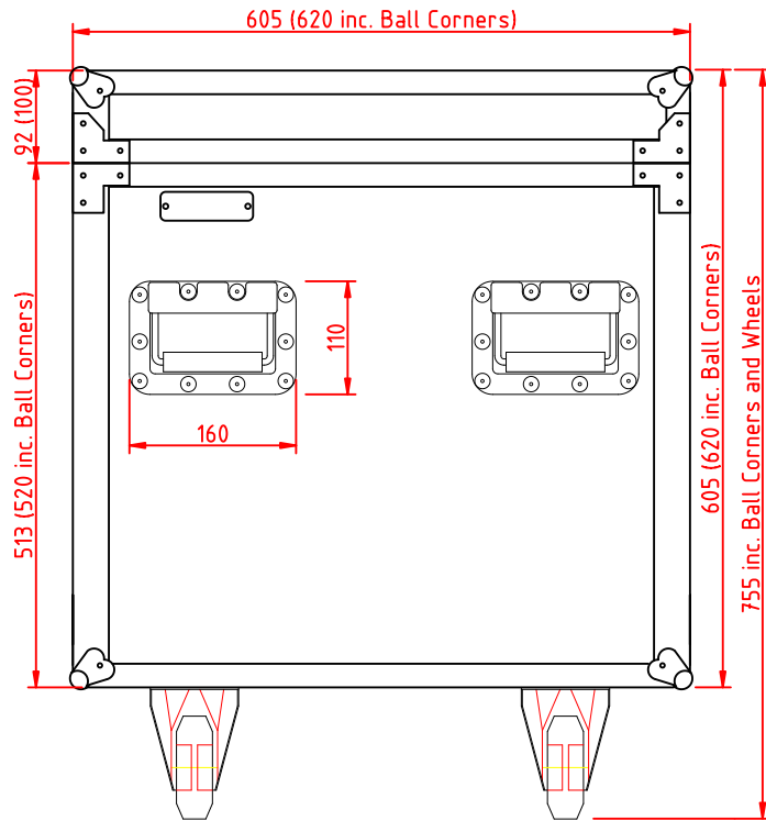
Cobra Case - FC33 Universal Tour Case Material: Plywood Dimensions in mm, may vary slightly
