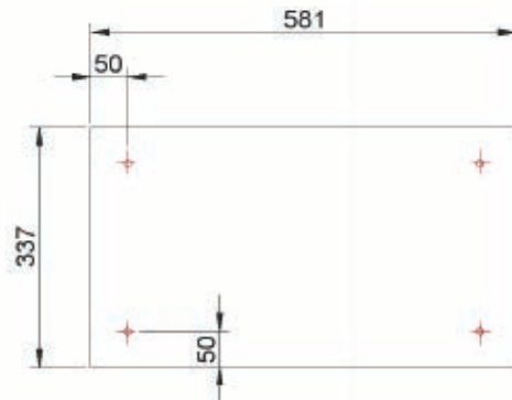
Cobra Case: FC191 Material: Ply Wood Dimensions in mm, May Vary Slightly.
