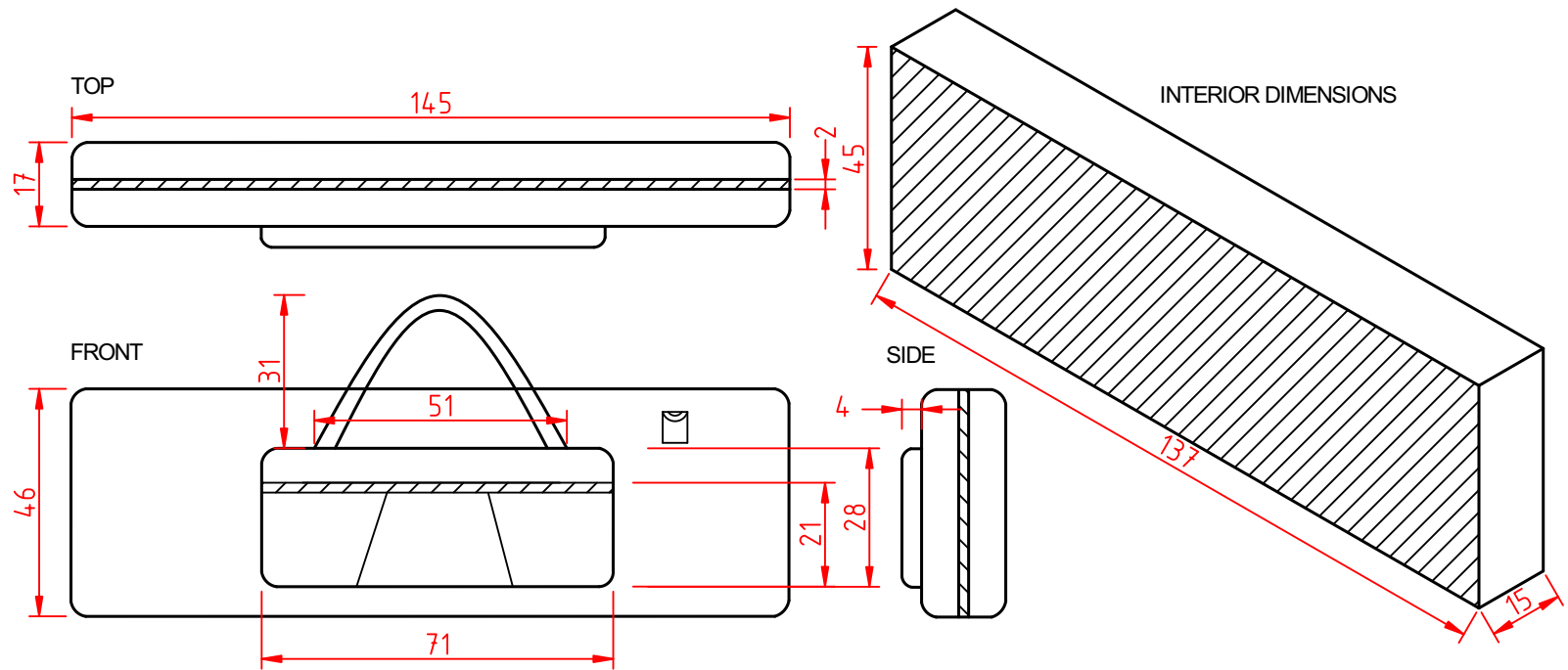
Cobra Case Keyboard Bag CC1052 Material: Polyester 600d Zips: No10 Dimensions in cm, may vary slightly
